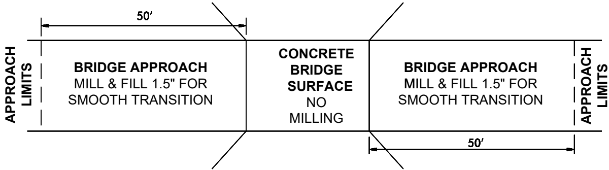
DETAIL FOR MAP # 6 / STRUCTURE # # 0225
