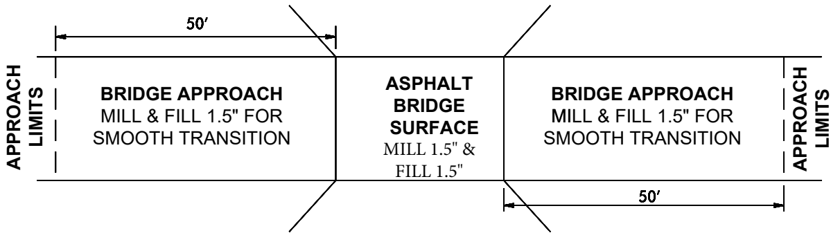
DETAIL FOR MAP # 2 & 5 / STRUCTURE # 0153 & 143
