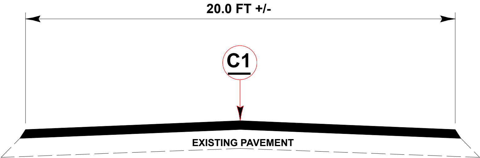
TYPICAL SECTION # 1 MAP(S) # 1 - 6
